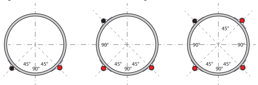
Fig. 12. Recommended ways to mount the cable lines.
