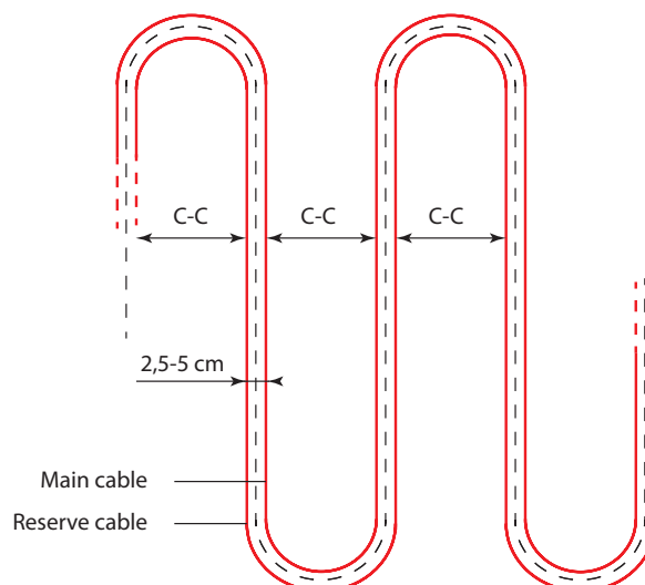
Fig. 4 – Main and reserve heating cables
